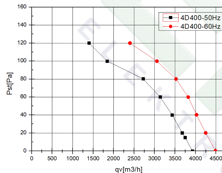
FLOW RATE CURVE (风量曲线) :
