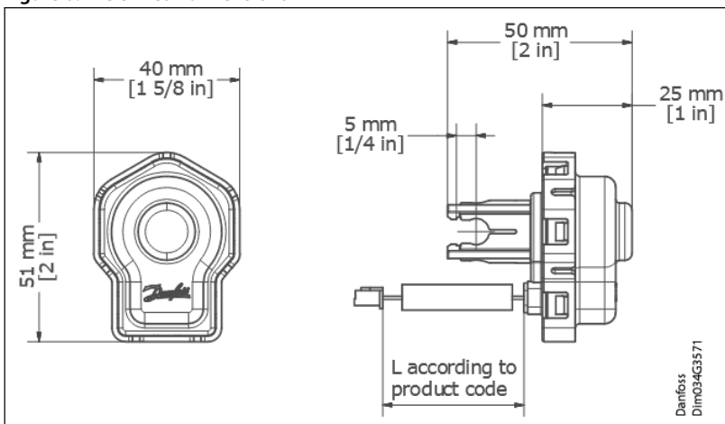
Figure 6: ETS 5M coil dimensions
