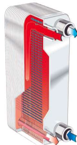
Condenser, showing flow principle.
