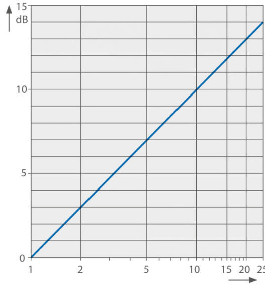
Fig. II: Addition of several sound sources
