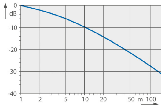
Fig. IV: Reduction of sound pressure level
