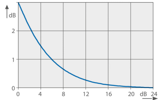
Fig. III: Sound sources of different levels
